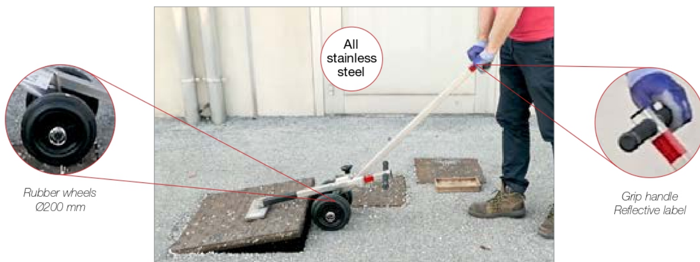
5400.25-03C Adapter for MR. OLIMPIA (400 kg)
