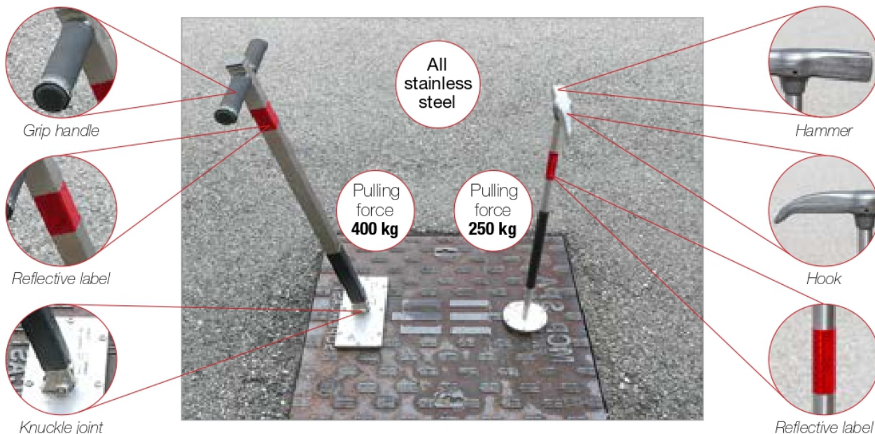
5400.25-03 Magnetic hoist MR. OLIMPIA (400 kg)
