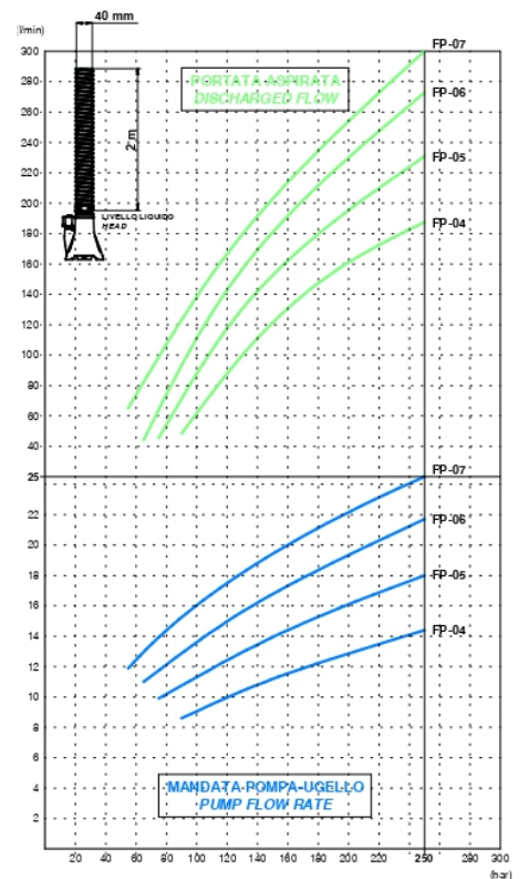
DN40 device: discharged flow and pressure according to the pump flow and size of nozzle (FP).
